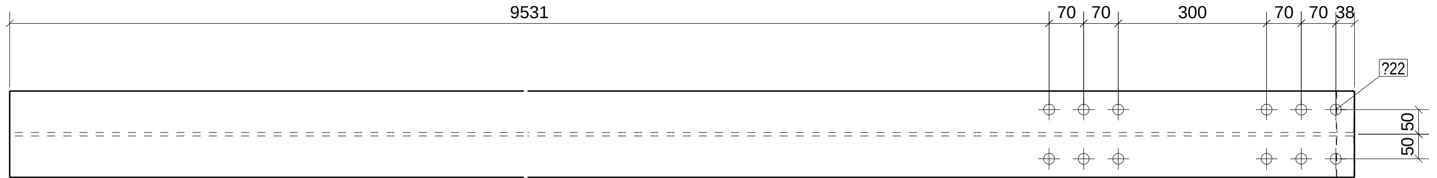
TOP VIEW
