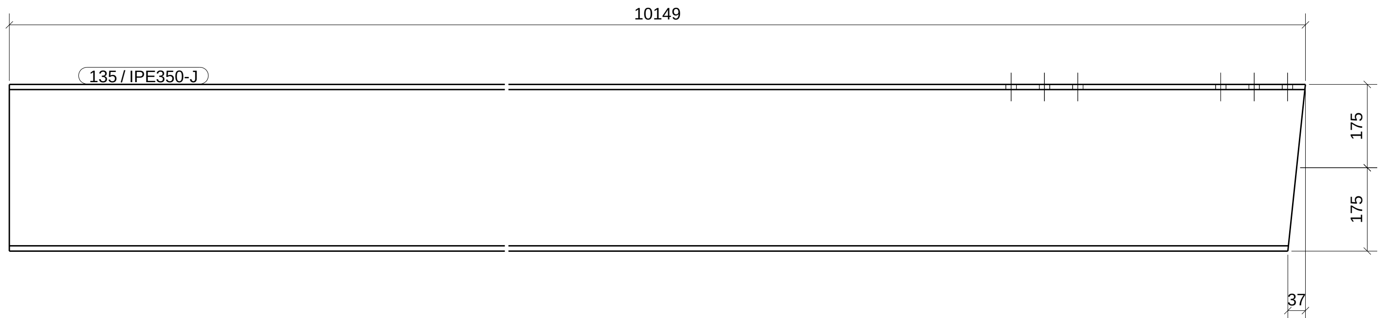
FRONT VIEW
